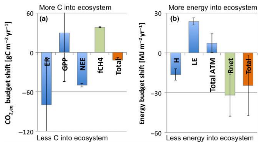
FIGURE 4 Shifts in annual budgets of carbon and energy following drainage. (a) Shifts in annual carbon budget components, converted to [\text{CO}_{2,\text{eq}}] , as a consequence of long-term drainage disturbance at the Ambolikha observation site (ER, ecosystem respiration; GPP, gross primary productivity; NEE, net ecosystem exchange as the sum of ER and GPP; f\text{CH}_4 , methane flux). (b) Shifts in annual energy budget components following drainage (H, sensible heat flux; LE, latent heat flux; total ATM, vertical energy exchange with the atmosphere as the sum of H and LE; Rnet, net radiation energy input)
