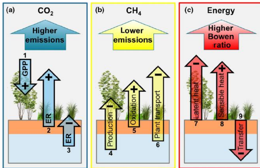
FIGURE 3 Conceptual overview on positive and negative feedbacks to climate change linked to permafrost drainage effects. (a) \text{CO}_2 : The strong increase in ecosystem respiration from shallow soils (2) dominates over increases in photosynthetic uptake (1) and minor decreases in respiration from deeper soil (3), causing increased net \text{CO}_2 emissions; (b) \text{CH}_4 : a decreased production in colder deep soils (4) in combination with higher oxidation in warmer and aerobic shallow soils (5) and less efficient plant transport (6) contribute to a strong decrease in \text{CH}_4 emissions; (c) energy: the reduction in latent heat fluxes (7) is almost balanced by increases in sensible heat (8), therefore shifting Bowen ratios. Reduced soil heat transfer (9) contributes to cooling permafrost soils
